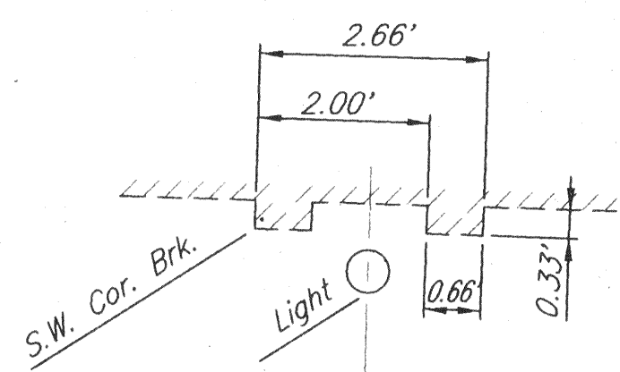
TYPICAL BRICK PROJECTION ALONG SOUTH PROPERTY LINE
