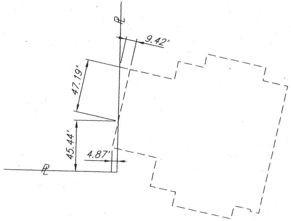
ENCROACHMENT DETAIL C SEARS AUTO CENTER BLDG.
