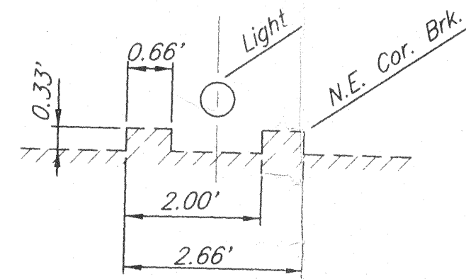
TYPICAL BRICK PROJECTION ALONG NORTH PROPERTY LINE
